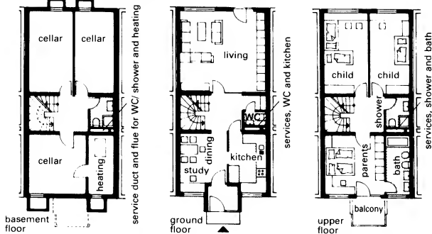
5 Terraced houses: all services contained in one duct
